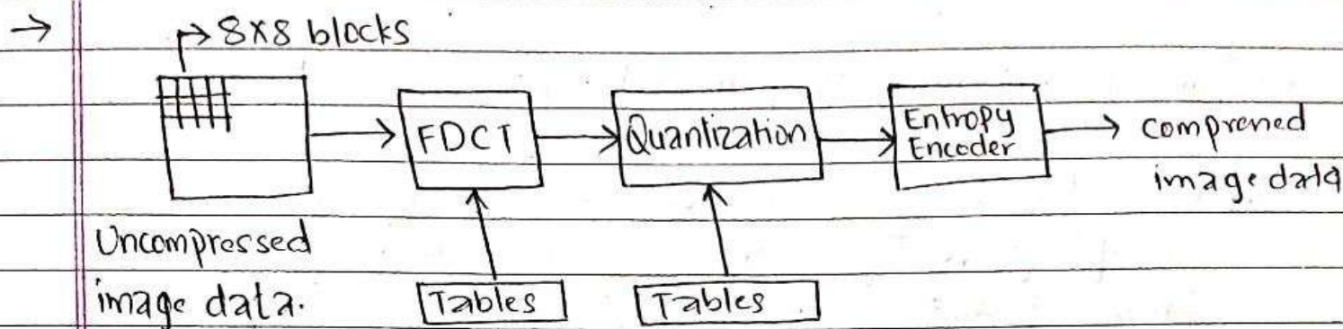
Fig: Lossy Sequential DCT based mode.
